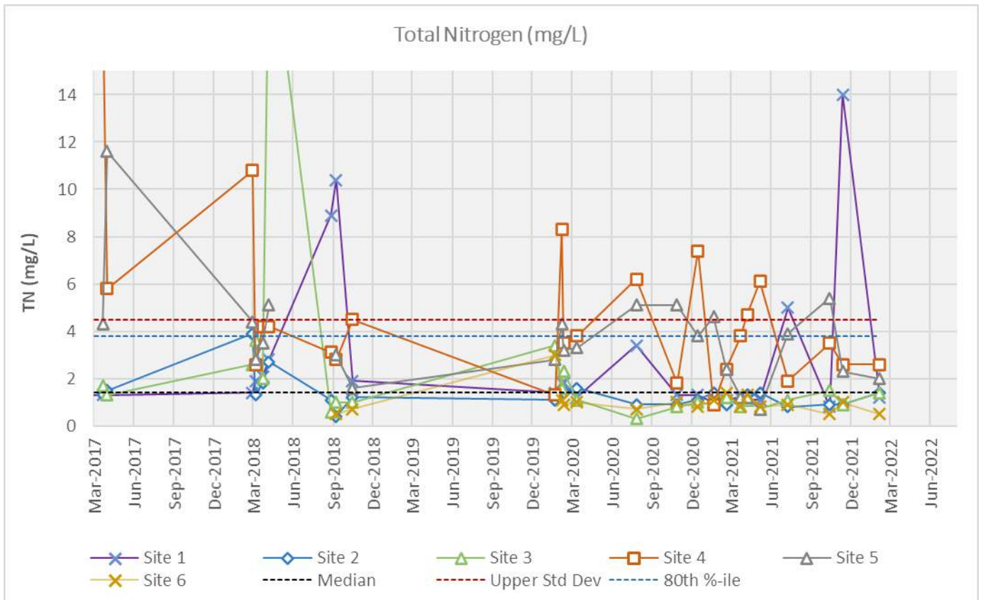
Figure 11. Total Nitrogen (TN) sampling time series.
