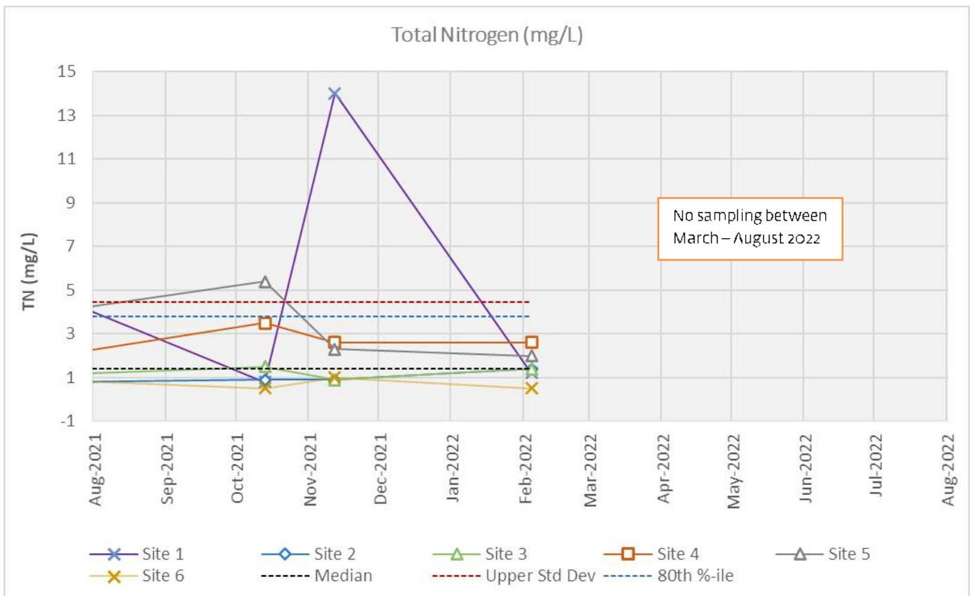
Figure 6. Total Nitrogen (TN) sampling time series.
