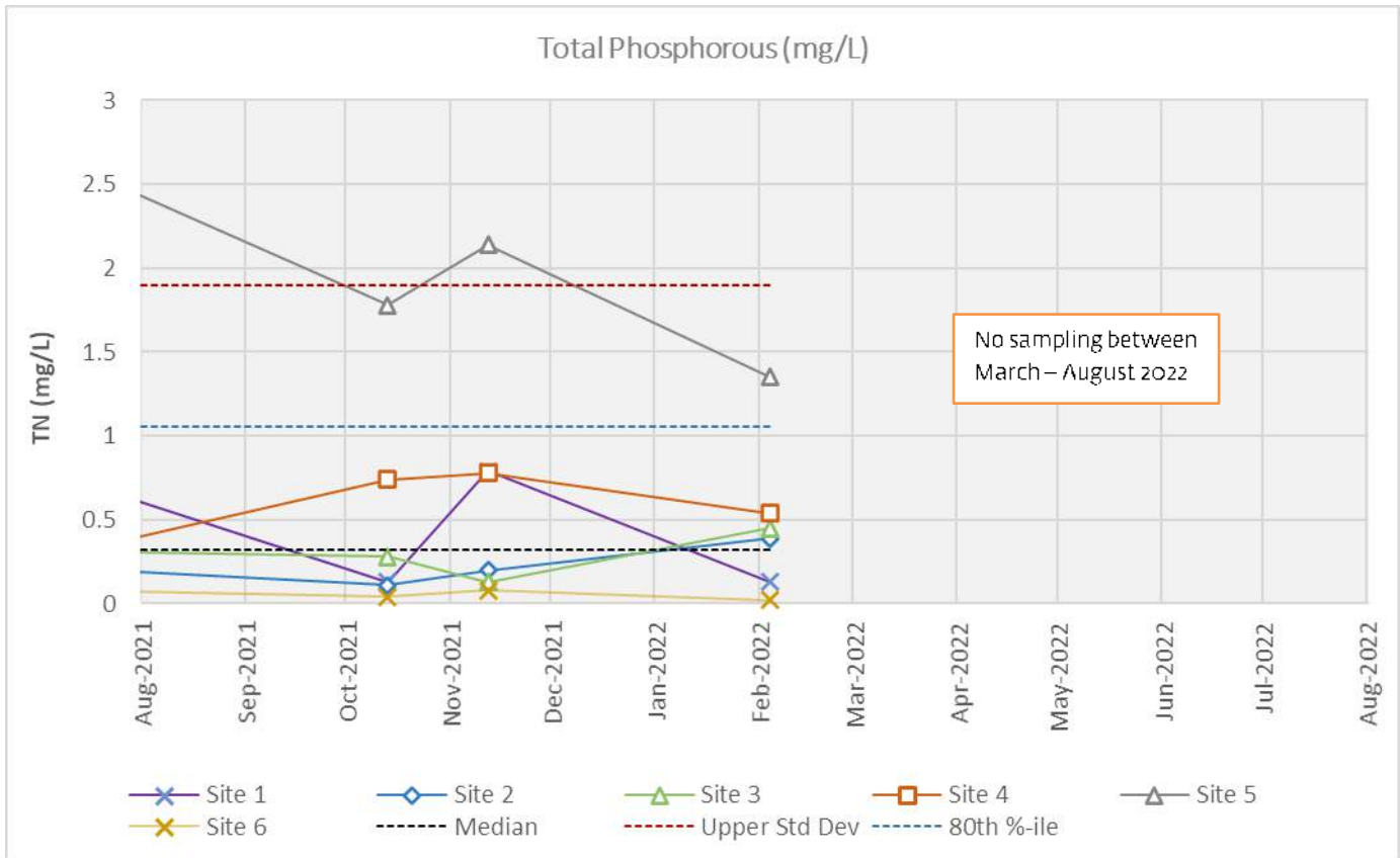
Figure 5. Total Phosphorous (TP) sampling time series.
