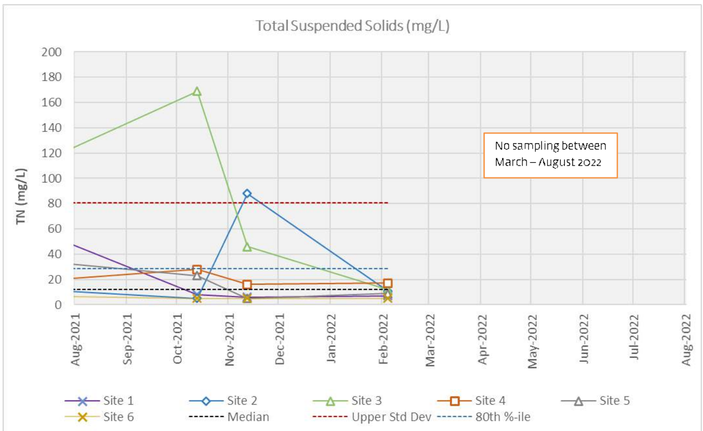
Figure 4. Total Suspended Solids (TSS) sampling time series.
