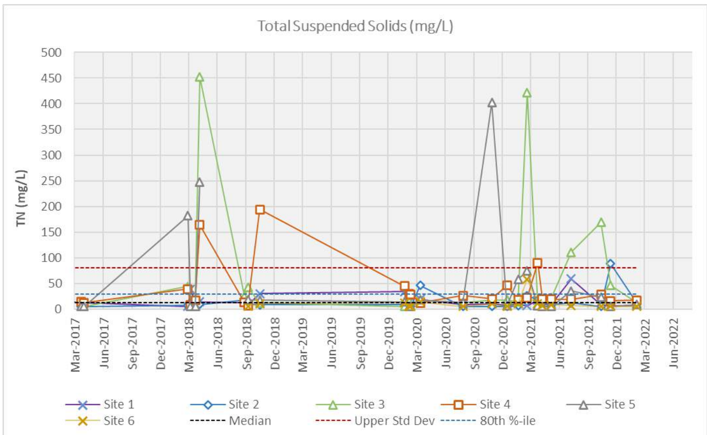
Figure 9. Total Suspended Solids (TSS) sampling time series.
