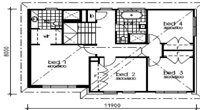
FIRST FLOOR PLAN EMERALD 24 - TRADITIONAL FACADE - RH
