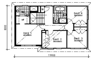
FIRST FLOOR PLAN EMERALD 24 - TRADITIONAL FACADE - RH
