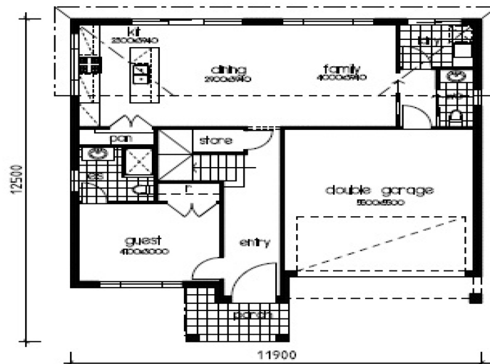
GROUND FLOOR PLAN EMERALD 24 - TRADITIONAL FACADE - RH
