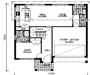
GROUND FLOOR PLAN EMERALD 24 - TRADITIONAL FACADE - RH
