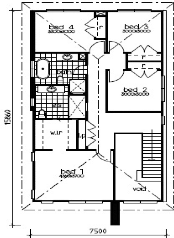
FIRST FLOOR PLAN RUBY 25M 2 - VOGUE FACADE - LH
