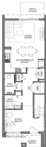
GROUND FLOOR
