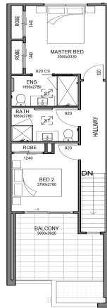
FIRST FLOOR
